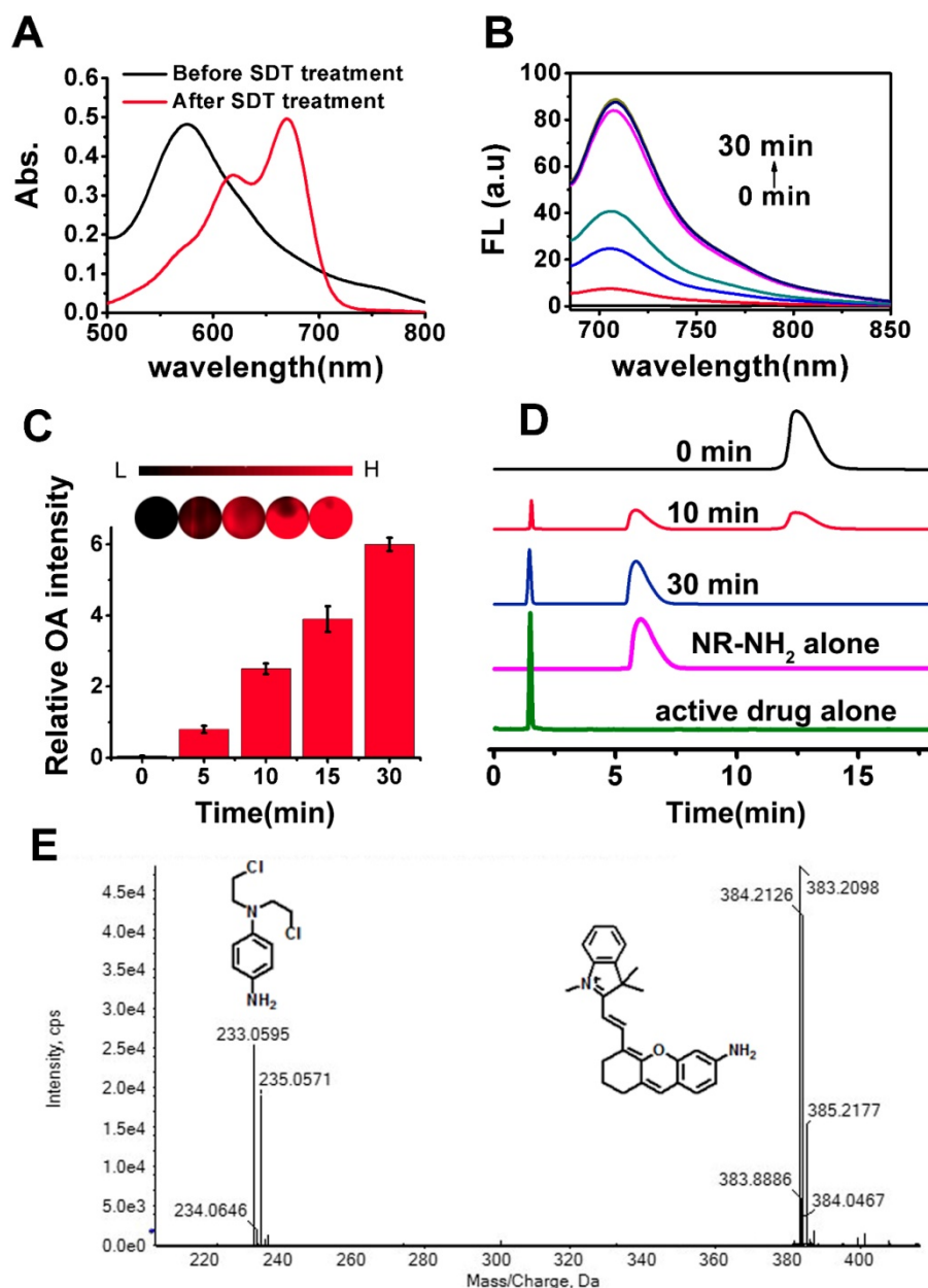
Figure 1. (A) Absorption spectra of NR-azo before and after treatment with SDT (100 \mu M). (B) Fluorescence spectra of NR-azo before and after treatment with MLM (50 \mu g/mL) and NADPH (cofactor for reductases, 100 \mu M) for different time (up to 30 minutes). (C) Optoacoustic response of NR-azo toward hypoxia (upon treatment with MLM). (D) HPLC profile for pure NR-NH 2 (Magenta line), the active drug (green line) and NR-azo upon treated with MLM for varied time. (E) HR-MS spectrum of NR-azo upon treatment with MLM.
