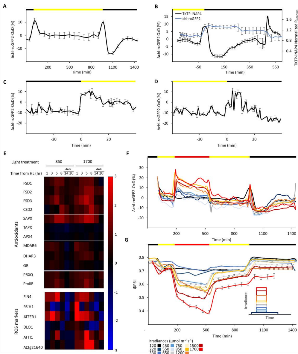
Figure 2: Diurnal changes in the degree of chl-roGFP2 oxidation under normal and high-light growth conditions. chl-roGFP2 fluorescence was monitored over a 24-hour period and chl-roGFP2 OxD values were calculated. Oxidation values were normalized to steady state values (as observed during the day at a constant light intensity of 120 \mu\text{mol m}^{-2} \text{s}^{-1} ). Horizontal bars above graphs show light (yellow) and dark (black) periods. (A) Changes in chl-roGFP2 OxD over time from the light onset under normal light conditions. Values are presented as means of 8 plants \pm SE. (B) Changes in chl-roGFP2 OxD and normalized R400/485 of TKTP-iNAP4 over time during the nighttime. Results of TKTP-iNAP4 were normalized using the pH control sensor (TKTP-iNAPc) according to Lim et al. (2020) and values are presented as means of 12 plants \pm SE. (C) Oxidation and rereduction of chl-roGFP2 during dark-to-light transitions. Values are shown as means of 16-24 plants \pm SE. (D) Oxidation and rereduction of chl-roGFP2 during light-to-dark transitions, shown as means of 16-45 plants \pm SE. (E) Temporal changes in expression of chloroplast-targeted genes encoding antioxidant proteins and established ROS markers. Gene expression levels in plants exposed to HL (850 or 1700 \mu\text{mol m}^{-2} \text{s}^{-1} ) were normalized to the gene expression in plants grown under normal light conditions (120 \mu\text{mol m}^{-2} \text{s}^{-1} ) at each indicated time point after start of the HL illumination. All data are displayed as the log 2 ratio. The red and blue colors represent high or low expression levels, respectively. (F) Diurnal changes in chl-roGFP2 OxD in wild type (WT) plants exposed to HL. For each treatment, between 21 and 24 plants, divided into 3 independent plates, were tested. For clear presentation of the redox changes of roGFP2 over time, a “sliding window” approach for the data along the x-axis was taken, in which each data point represents the average of three plates ( n=3 ). roGFP2 data were acquired using the chl-TKTP-roGFP2 line. Inset: Experimental design for the HL experiments. For a depiction of absolute roGFP2 OxD values and illustration of SE values see Supp.Fig.15 and Supp.Fig.16. (G) Diurnal changes in chl-roGFP2 \Phi\text{PSII} values in plants exposed to the same conditions as in (D). \Phi\text{PSII} values were derived from chlorophyll fluorescence analysis and represent means of 12 plants \pm SE.
