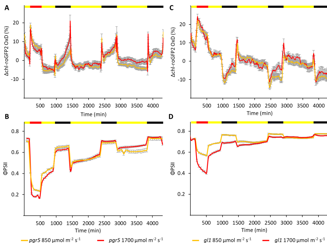
Figure 5: Diurnal changes in chl-roGFP2 OxD and \Phi_{PSII} during one day of high-light regime followed by two days of normal light conditions in pgr5 and gl1 plants. (A, C) Changes in chl-roGFP2 OxD over time from the experiment onset. chl-roGFP2 fluorescence was monitored throughout the experiment and chl-roGFP2 OxD values were calculated. Oxidation values were normalized to steady state oxidation levels. Each treatment involved 32 plants divided into four independent plates that were consolidated in a “sliding window” (n=4) display. Values represent means \pm SE for pgr5 (A) and gl1 (C). roGFP data were acquired using the chl-PRX ATP -roGFP2. (B) \Phi_{PSII} over time from the experiment onset. \Phi_{PSII} values were derived from chlorophyll fluorescence measurements and represent means of 12 plants \pm SE for pgr5 (B) and gl1 (D). The color bar denotes the light conditions: black – night, yellow – normal light, red – high light
