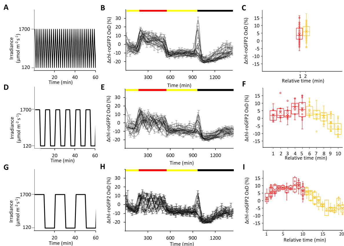
Figure 3: Diurnal changes in chl-roGFP2 OxD under fluctuating light conditions. (A, D, G) Light irradiance during time over a 60-min period, extracted from the fluctuating light phase, is presented for the applied intervals of 1, 5 and 10 min. (B, E, H) Changes in chl-roGFP2 OxD values ( \Delta OxD) over time in Arabidopsis plants expressing chl-TKTP-roGFP2. After the start of the illumination period (yellow bar, 120 \mu\text{mol m}^{-2} \text{s}^{-1} for 3 h), the illumination regime was switched to fluctuating light alternating between HL ( 1700 \mu\text{mol m}^{-2} \text{s}^{-1} ) and normal light ( 120 \mu\text{mol m}^{-2} \text{s}^{-1} ) with different intervals. After 6 h fluctuating light (red bar), illumination continued continuously at 120 \mu\text{mol m}^{-2} \text{s}^{-1} for 7 h before the diurnal cycle ended with 8 h darkness (black bar). Oxidation values were normalized to steady state values (as observed during the day at constant light conditions of 120 \mu\text{mol m}^{-2} \text{s}^{-1} ). Each black line represents the oxidation dynamics recorded for an independent well plate which consists of 8 plants. Values represent means of these 8 plants \pm SE. (C, F, I) \Delta OxD as a function of relative time (min) within each fluctuating light cycle. Values measured during the HL ( 1700 \mu\text{mol m}^{-2} \text{s}^{-1} ) phases within each light cycle are presented in red. Values measured during the phases with normal light intensities ( 120 \mu\text{mol m}^{-2} \text{s}^{-1} ) during each light cycle are presented in yellow. The presented box spans the interquartile range, and whiskers represent the minimum and maximum values (not including outliers). The median and mean of at least six plants are marked by a vertical line and x sign inside the box, respectively.
