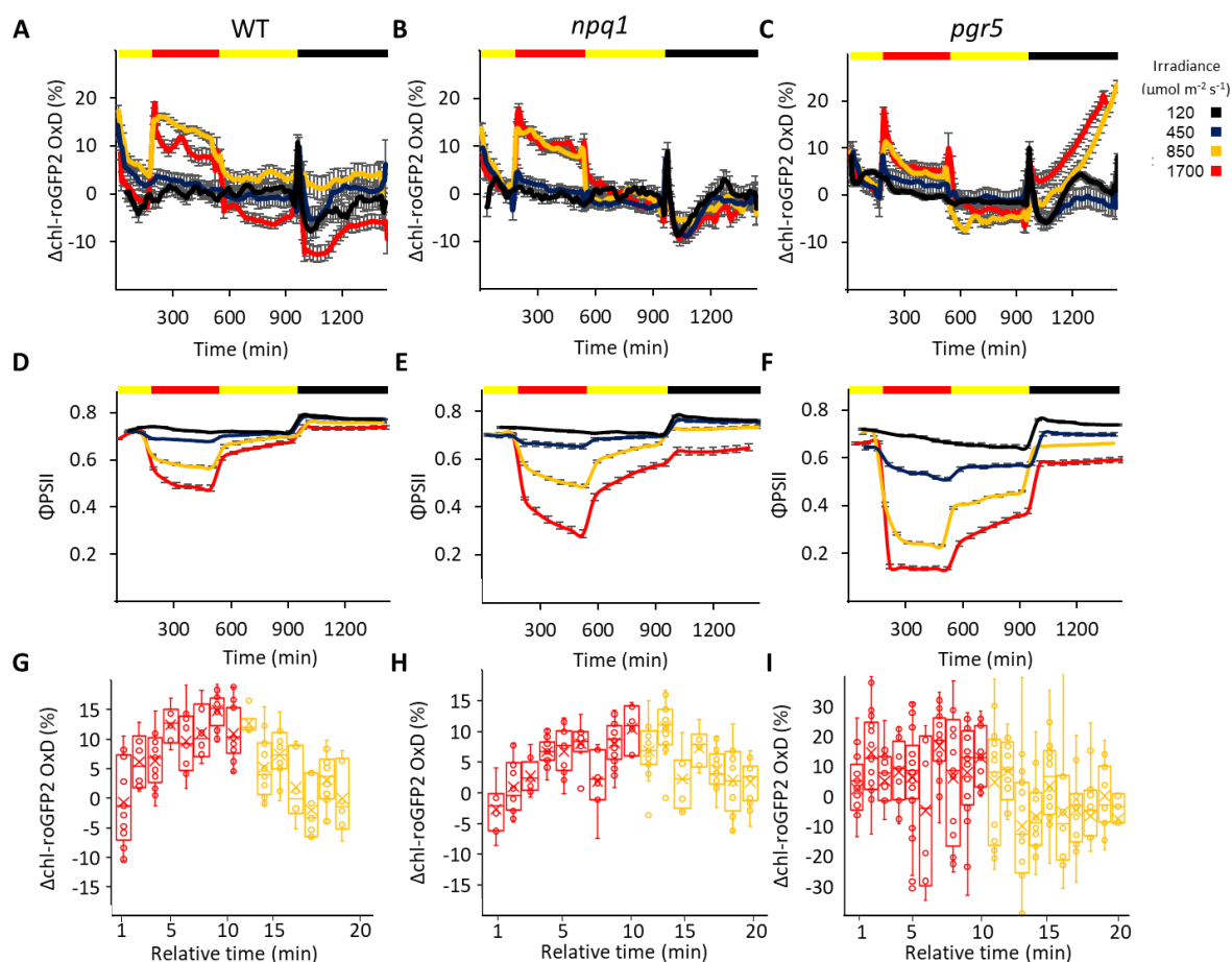
Figure 4: Diurnal changes in chl-roGFP2 OxD and \Phi PSII under high-light and fluctuating light conditions in mutants with defects in photoprotective mechanisms. (A, B, C) Daily changes in chl-roGFP2 OxD under different light regimes in WT (A), npq1 (B) and pgr5 (C) plants expressing chl-PRXa TP -roGFP2. The respective absolute ratio (400/485) data are provided in Supp. Fig.17. Oxidation values were normalized to steady state oxidation levels under normal growth light. The illumination regime was: 3 h normal light (yellow bar, 120 \mu\text{mol m}^{-2} \text{s}^{-1} ), followed by 6 h HL (red bar, intensities as indicated by line color), 7 h normal light (120 \mu\text{mol m}^{-2} \text{s}^{-1} ) and 8 h darkness. Each treatment involved between 24 and 32 plants divided into four independent plates that were consolidated in a “sliding window” ( n=4 ) display. Values represent means \pm SE. (D, E, F) \Phi PSII for WT (D), npq1 (E) and pgr5 (F) plants exposed to the same light regimes as in A, B and C. \Phi PSII values were derived from chlorophyll fluorescence measurements and represent means of 12 plants \pm SE. (G-I) Changes in chl-roGFP2 OxD during FL cycles with 10-min HL (1700 \mu\text{mol m}^{-2} \text{s}^{-1} ) and 10 min normal light (120 \mu\text{mol m}^{-2} \text{s}^{-1} ) for WT (G), npq1 (H) and pgr5 (I) plants. Values measured during the HL (1700 \mu\text{mol m}^{-2} \text{s}^{-1} ) phases within each light cycle are presented in red. Values measured during the phases with normal light intensities (120 \mu\text{mol m}^{-2} \text{s}^{-1} ) during each light cycle are presented in yellow. The presented box spans the interquartile range, and whiskers represent the minimum and maximum values (not including outliers). The median and mean of at least six plants are marked by a vertical line and x sign inside the box, respectively.
